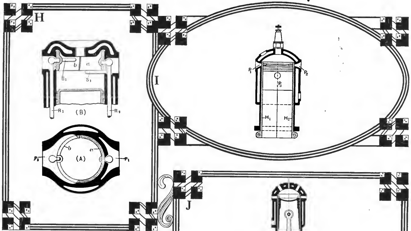
Fig. H—Sectional view of the Howard sliding sleeve valve motor utilizing a spherical split ring
